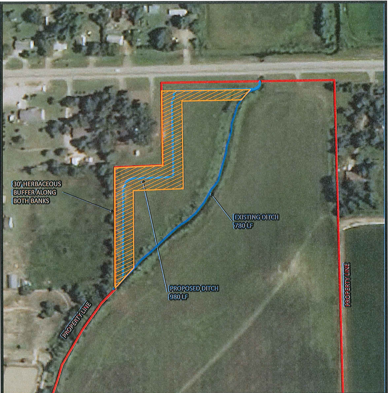
FIGURE 1. DITCH RELOCATION MAP Quality Grain Storage, LLC McDougal Farm at the Little Cache River Ditch
